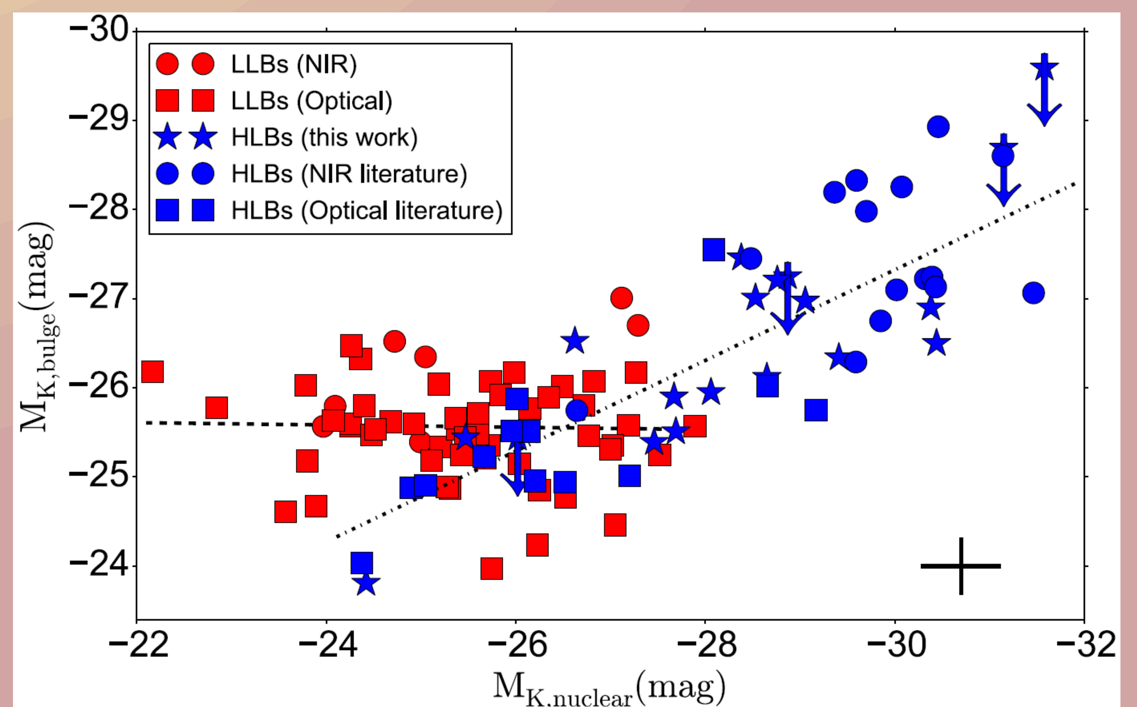
Figure 5. The correlation between nuclear and bulge magnitudes for high-luminosity blazars (HLBs) is consistent with a scenario where AGN activity results in positive feedback on the star formation rate wherein the more powerful the jet, the more significant the effect caused on its host galaxy.
