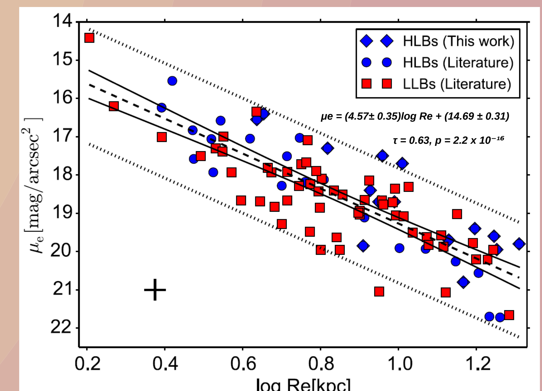
Figure 4. The Kormendy relation. We show the 95 per cent prediction bands (dotted lines) and the 95 per cent confidence intervals (solid lines). A typical error bar is shown in the lower left corner.
